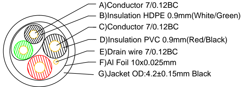
28+28AWG USB Cable Spec.
