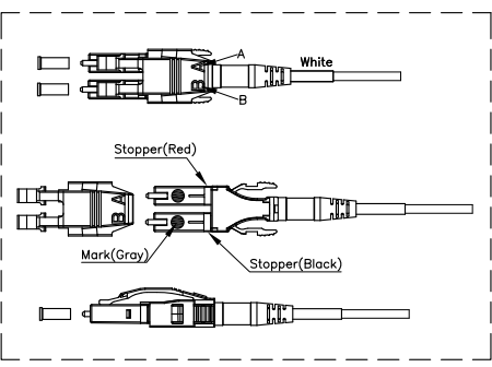
Polarity Twist LC Connector(SCALE 1/2)
