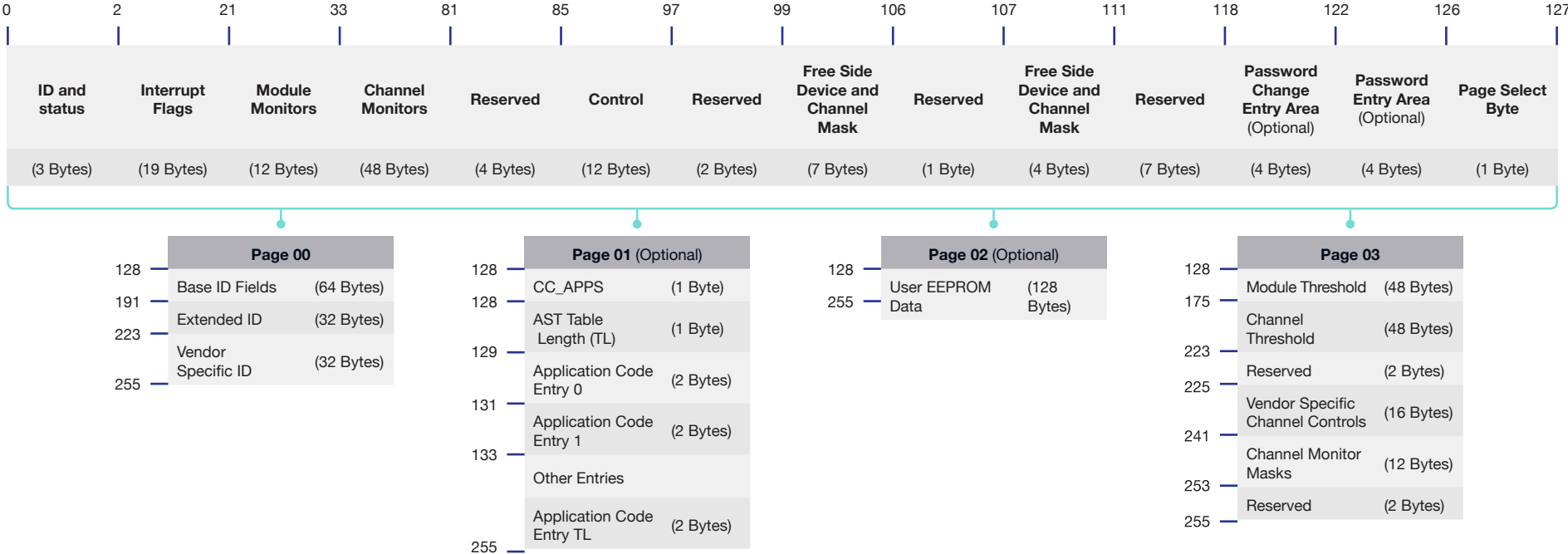
Figure 3. QSFP28 Memory Map
