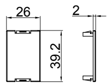
Blank module cover 1PC
