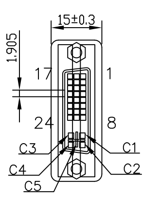
DVI 29F(NICKEL PLATED)
