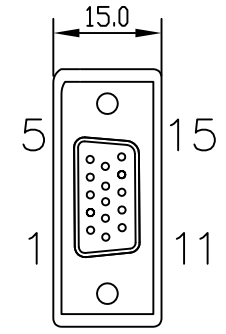
HD 15M(NICKEL PLATED)
