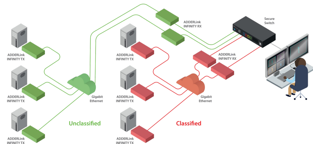
Fig. 3: When combined with an Adder matrix, a secure KVM switch provides the user with instant switching between larger groups of computers while retaining isolation. When accessing different security networks, an air gap must be maintained.
