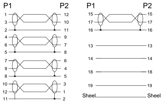
Wire method
