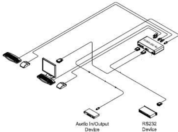
Figure 3– Connection of Receiver
