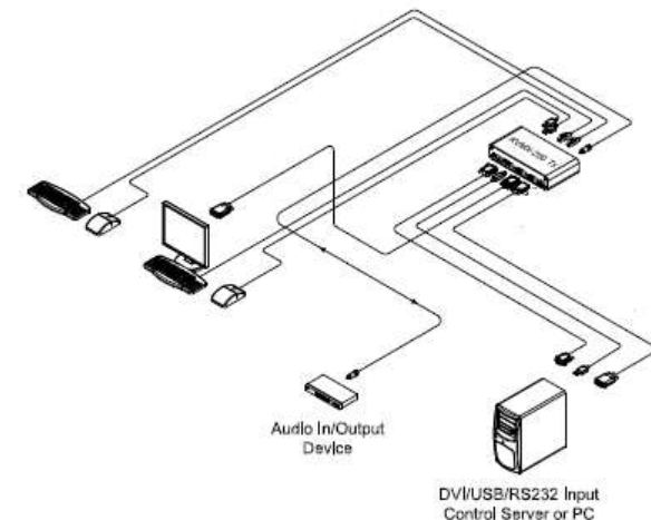
Figure 2– Connection of Transmitter
