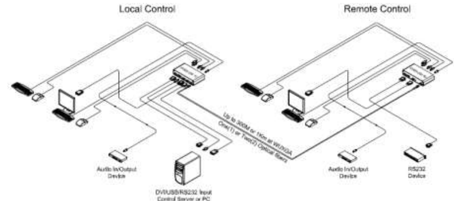
Figure 1– Connection Diagram
