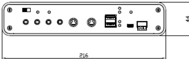
Transmitter
